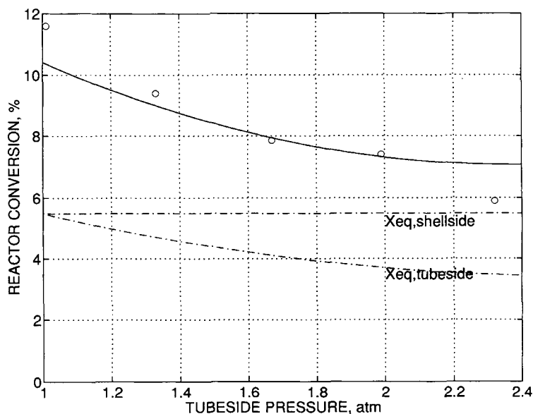
FIG. 8 Conversion vs pressure for dense feed, F_r = 1.0 , \tau = 2 s, T = 550^\circ\text{C} .
